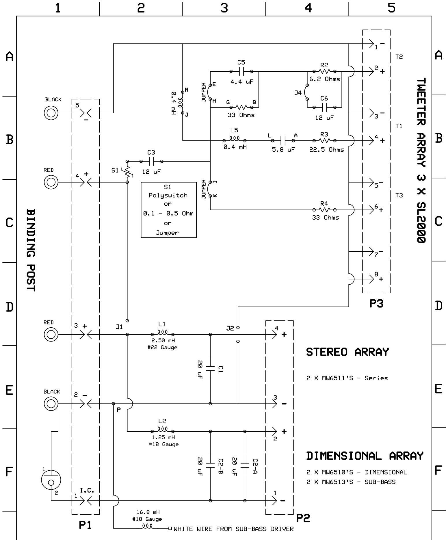
Custom SDA SRS 2.3 PCB Schematic
